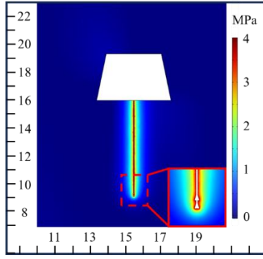
(a) grouting time 4 min
